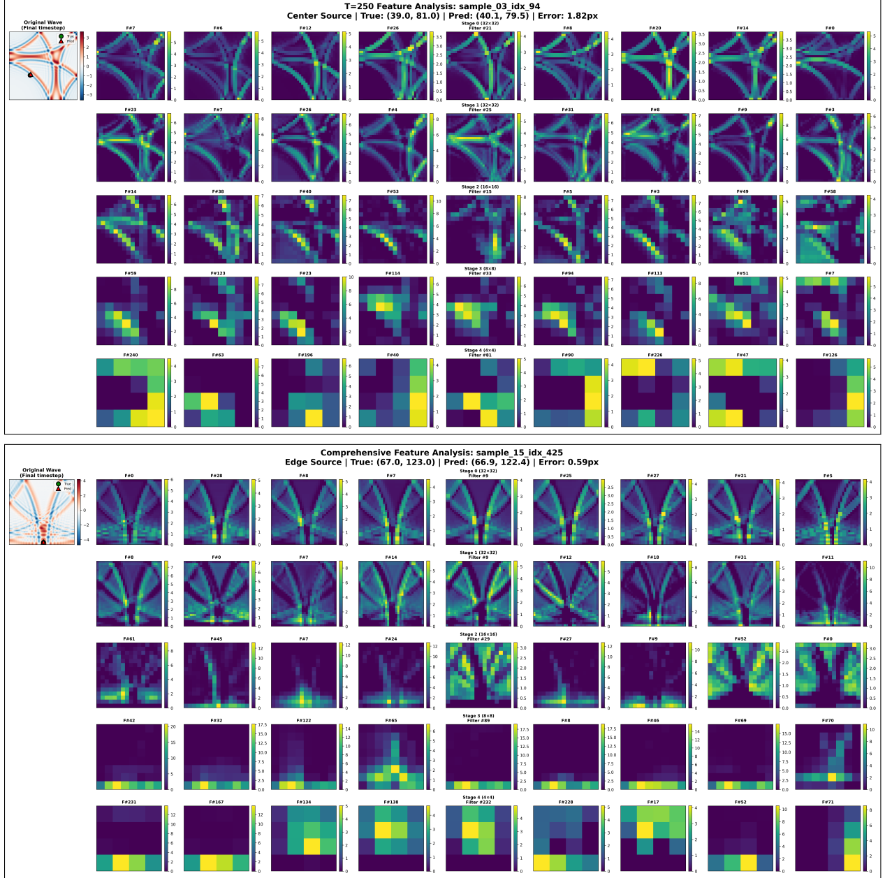
Figure 8: Feature maps for representative samples ( T=250/T=500 ), each image is the output of a specific filter, images from the same row are from the same layer.
